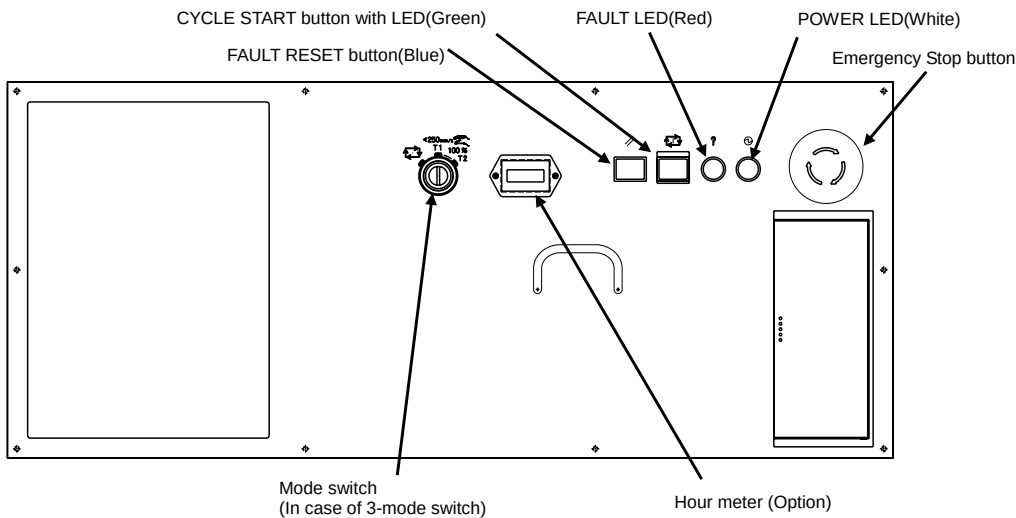
Fig.2 R-30iB/R-30iB Plus B-cabinet symbol operator's panel
