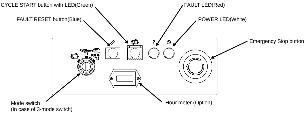
Fig.1 R-30iB/R-30iB Plus A-cabinet symbol operator's panel
